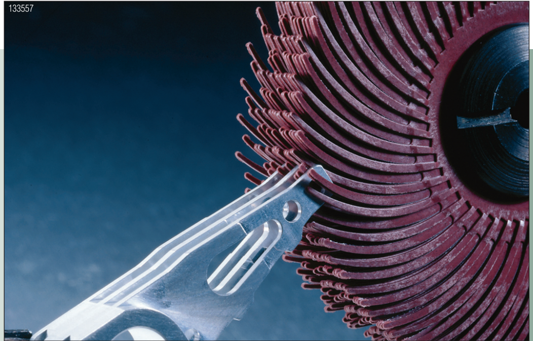
3" Radial Bristle Disc, thin bristle, grade 220, deburring and finishing aluminum internal hard drive part.
